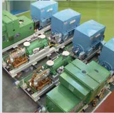
Ring Section Boiler Feed Pump Staythorpe C CCPP UK, 1x1,500MW
