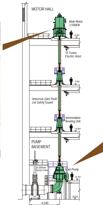
Main Sewage Pumps 18,720m 3 /h - 37.3m - 2,500kW - 8units
